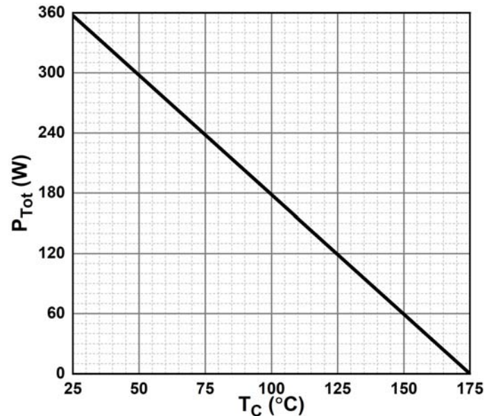
Figure 6. Power Derating
