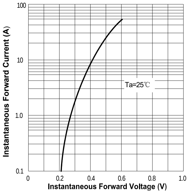
FIG.3: Forward Voltage
